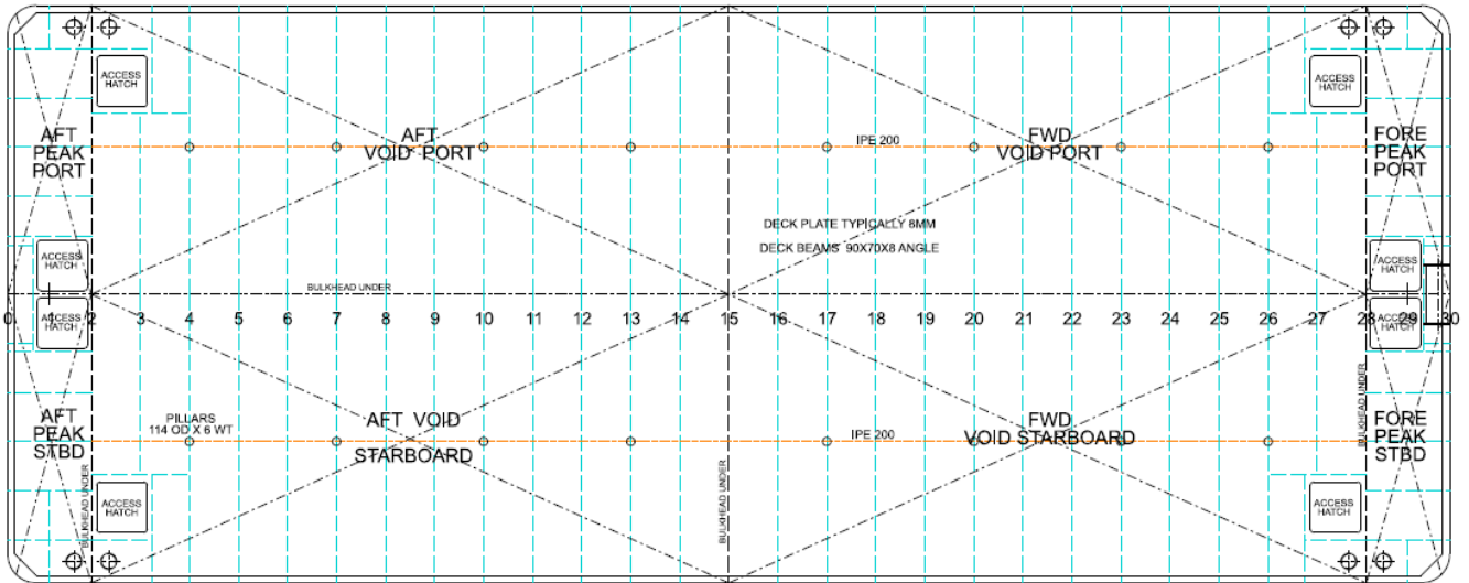
PLAN ON MAIN DECK
